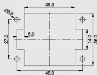
面板安装开孔图 Panel cut out
